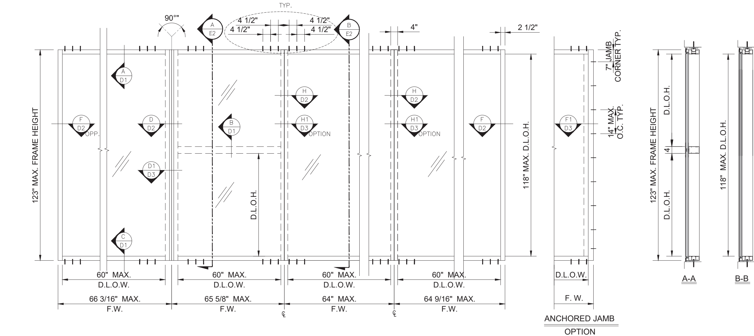
TYPICAL ELEVATION 4" UNREINFORCED MULLION
