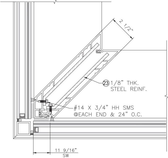
CORNER (C1)
