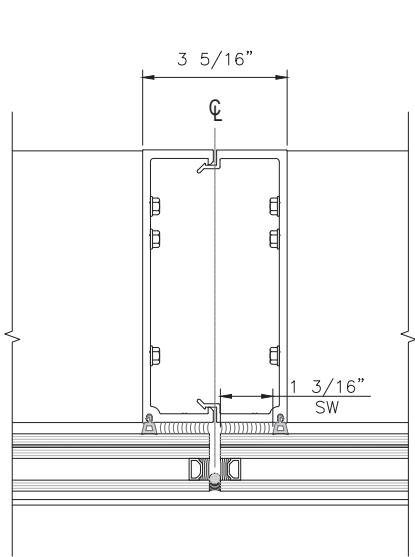
MULLION (M1)
