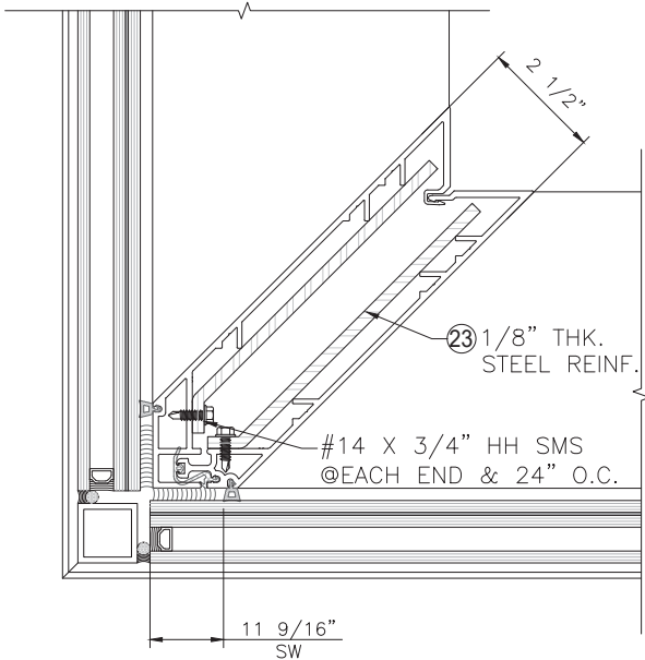
CORNER (C1)
