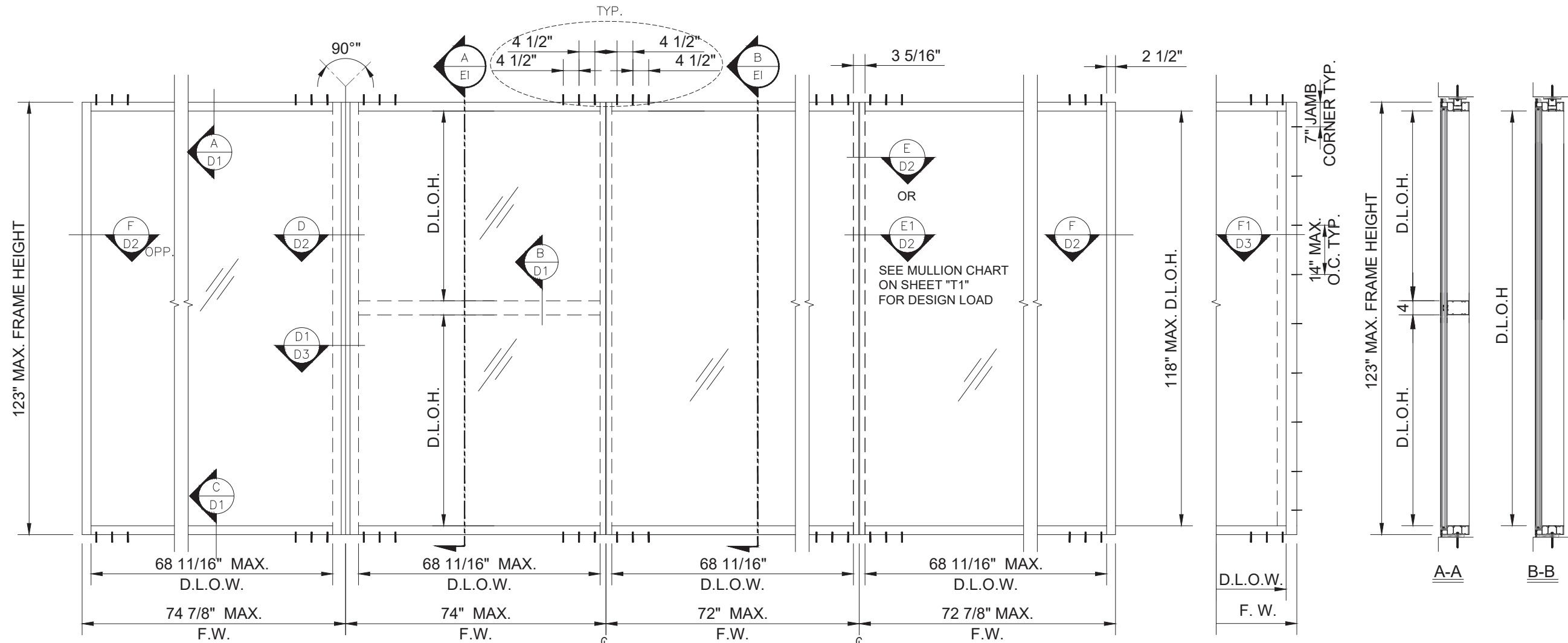
ANCHORED JAMB OPTION
