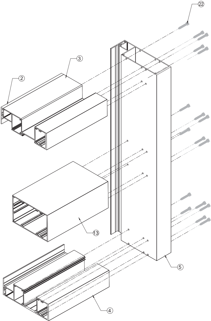
FRAME ASSEMBLY ISOMETRIC VIEW
