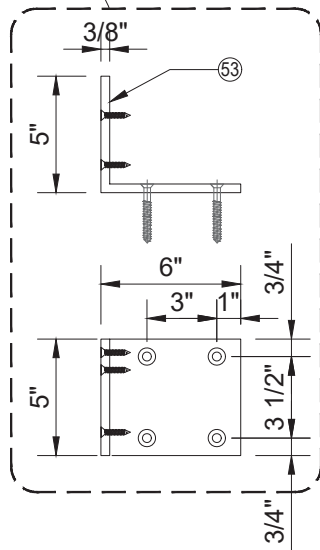
TYPICAL ANCHOR DETAIL
