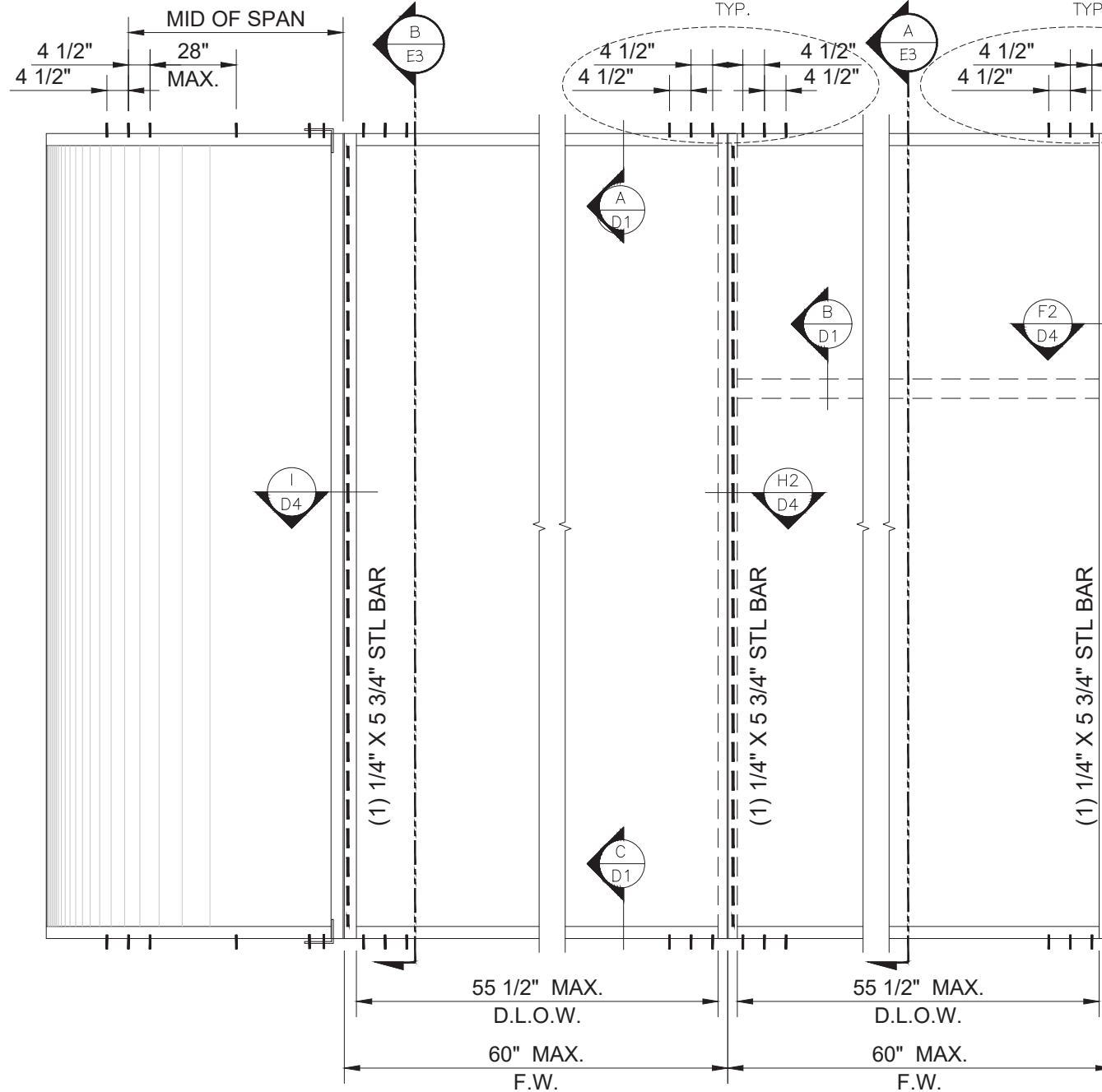
TYPICAL ELEVATION 4" REINFORCED MULLION
