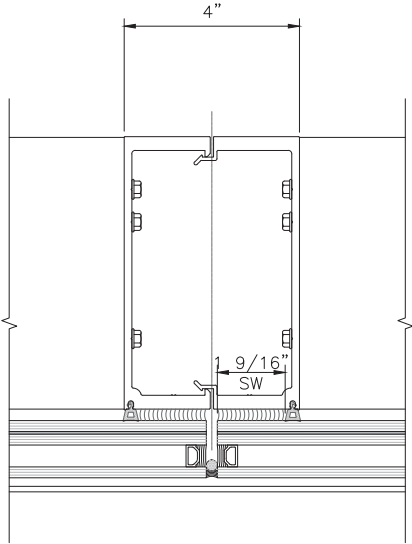
MULLION (M3)
