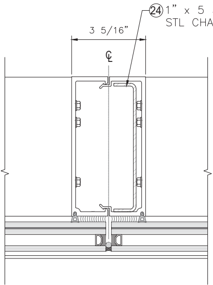
MULLION (M2)
